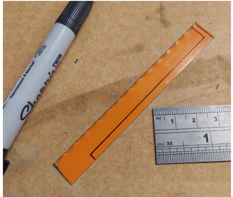
Figure 1 ♦ Using a thin permanent marker and a ruler to mark out our flat tension wrench design
