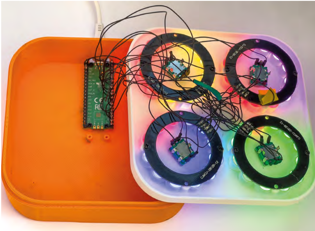
Figure 2 ♦ The box contains mounting pillars for a second Pico in case two devices were required: one to scan the encoders and another to send the MIDI messages. Fortunately, it turns out that a single Pico can handle both tasks quite happily
