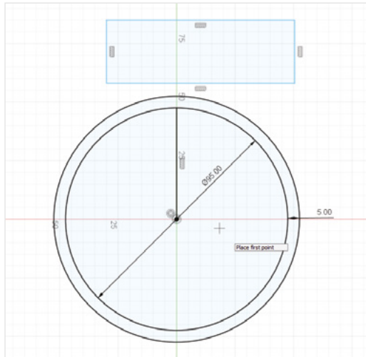
Figure 2 ◆ When adding the symmetry constraint, select the two features you want to be symmetrical before selecting the feature that will represent the line of symmetry
