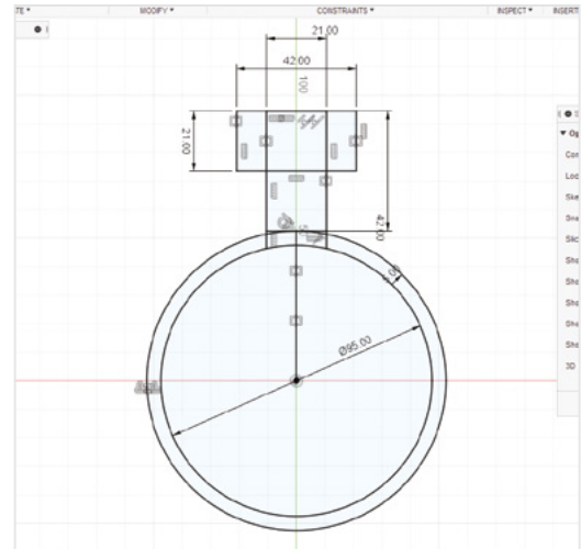
Figure 3 ◆ The finished sketch with all constraints and dimensions. Notice the small lines drawn to connect the ring to the rectangle
