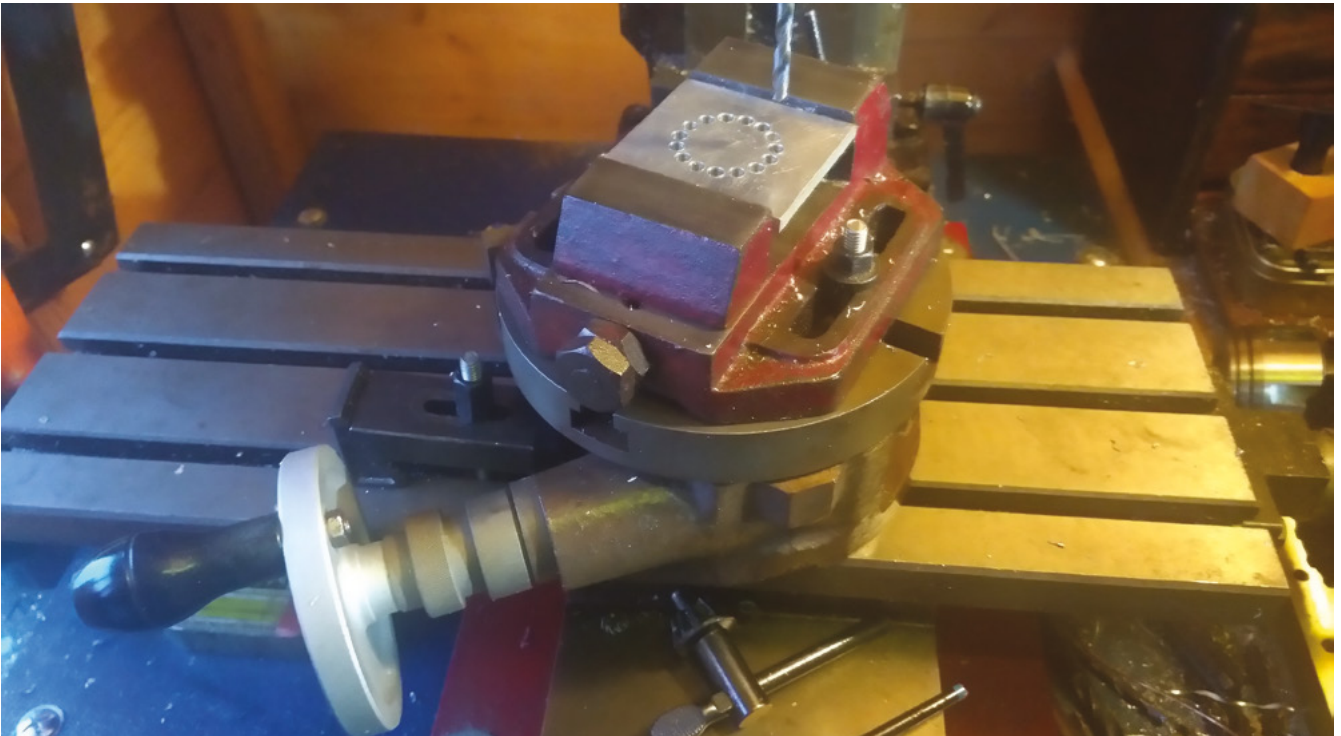
Figure 4 ♦ A rotary table can be used to index workpieces in various ways – in this instance to drill a circle of equidistant holes
