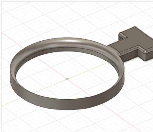
Figure 5 ♦ Select an edge and click on the Fillet button from the toolbar at the top of your screen. An arrow will appear on your model; drag it left and right to smooth the selected edge(s)
